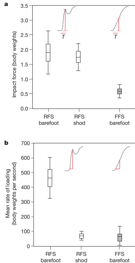
Figure 2 | Variation in impact transients. a, b , Magnitude ( a ) and rate of loading ( b ) of impact transient in units of body weight for habitually shod runners who RFS (group 1; open boxes) and habitually barefoot runners who FFS when barefoot (group 3; shaded boxes). The rate of loading is calculated from 200 N to 90% of the impact transient (when present) or to 6.2 \pm 3.7\% (s.d.) of stance phase (when impact transient absent). The impact force is 0.58 \pm 0.21 bodyweights (s.d.) in barefoot runners who FFS, which is three times lower than in RFS runners either barefoot ( 1.89 \pm 0.72 bodyweights (s.d.)) or in shoes ( 1.74 \pm 0.45 bodyweights (s.d.)). The average rate of impact loading for barefoot runners who FFS is 64.6 \pm 70.1 bodyweights per second (s.d.), which is similar to that for shod RFS runners ( 69.7 \pm 28.7 bodyweights per second (s.d.)) and seven times lower than that for shod runners who RFS when barefoot ( 463.1 \pm 141.0 bodyweights per second (s.d.)). The nature of the measurement (force versus time) is shown schematically by the grey and red lines. Boxes, mean \pm s.d.; whiskers, mean \pm 2 s.d.
