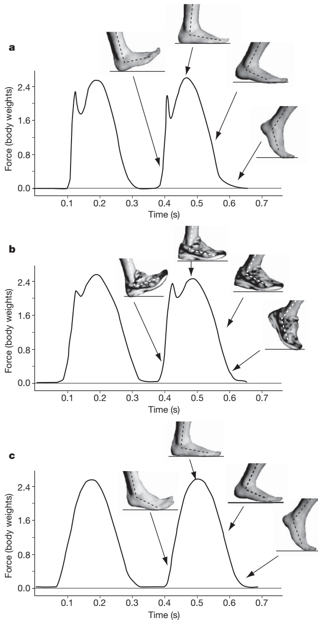
Figure 1 | Vertical ground reaction forces and foot kinematics for three foot strikes at 3.5 \text{ m s}^{-1} in the same runner. a , RFS during barefoot heel-toe running; b , RFS during shod heel-toe running; c , FFS during barefoot toe-heel-toe running. Both RFS gaits generate an impact transient, but shoes slow the transient's rate of loading and lower its magnitude. FFS generates no impact transient even in the barefoot condition.
